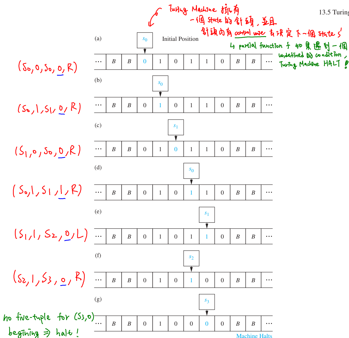
FIGURE 2 The steps produced by running T on the tape in Figure 1.
